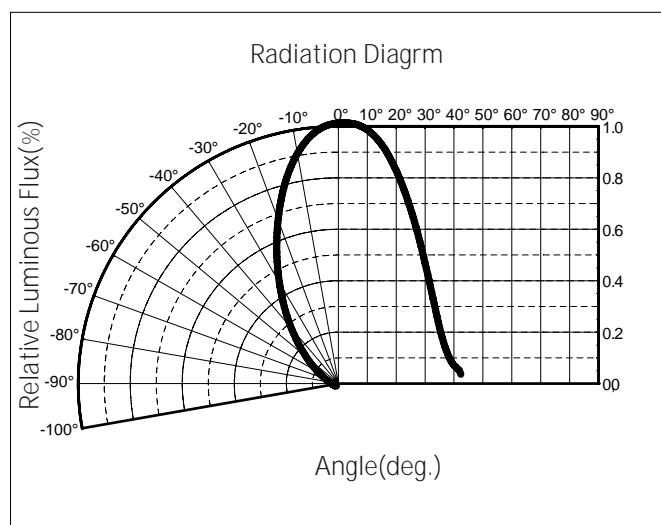
e) Beam Angle Characteristics ( T_j = 25^\circ\text{C} , I_F = 60\text{ mA} )
