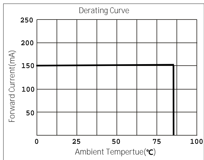
d) Derating Curve
